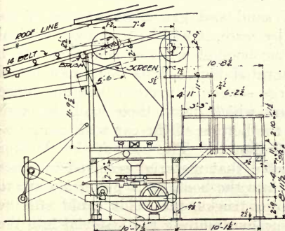
FIG. 23—SIDE ELEVATION AT MIXER END
